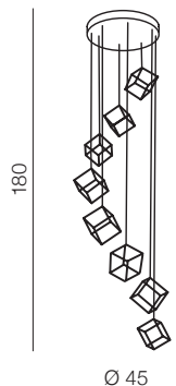
Strange 8 dimm LED
